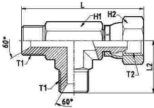
747 BSP 60° (ISO 228- PF)
