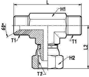
737 BSP 60° (ISO 228- PF)
